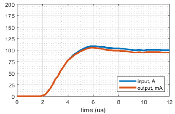
Figure 2: Typical step response (0 to 100 A, 36 A/μs R_M = 10 \Omega )
