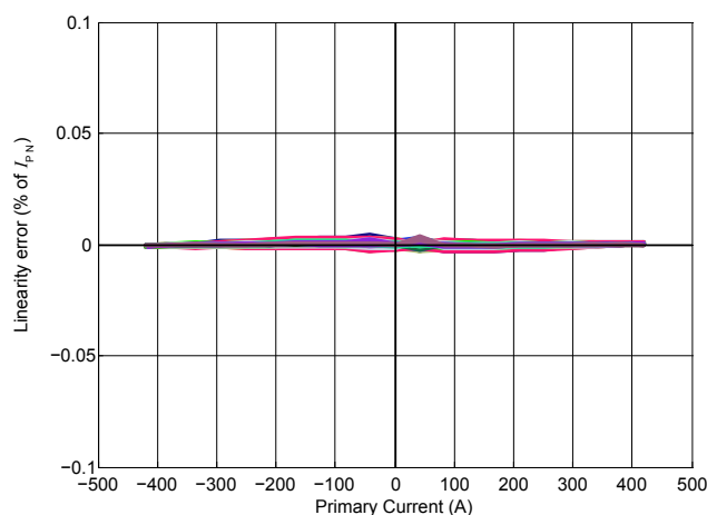
Figure 5: Linearity
