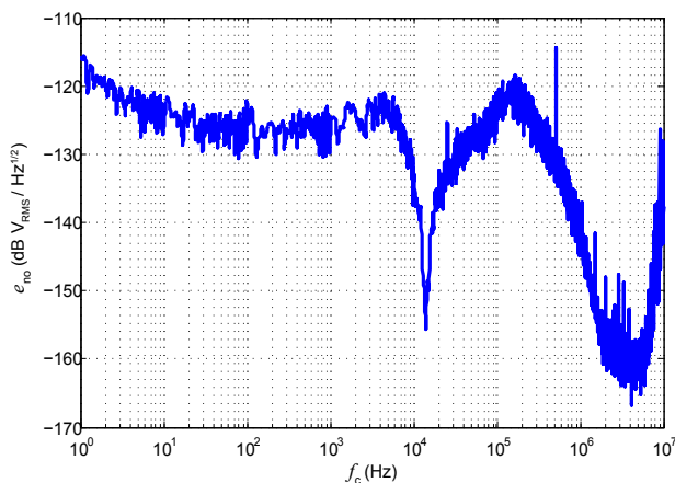
Figure 3: Typical output noise voltage spectral density e_{no} with R_M = 10 \Omega
