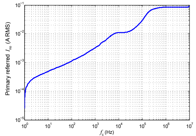
Figure 4: Typical RMS noise current referred to primary I_{no} with R_M = 10 \Omega
