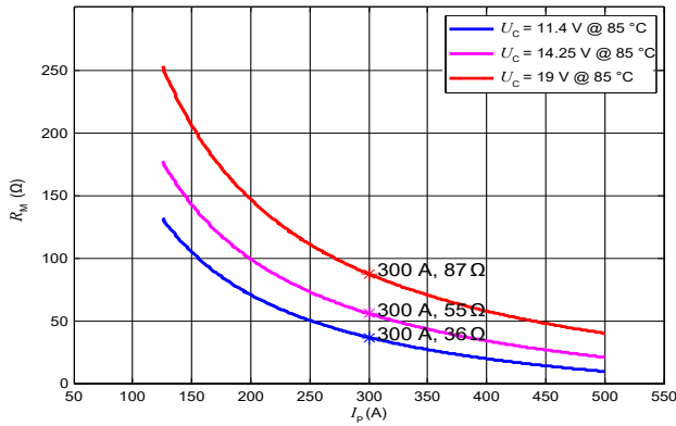
Figure 1: Maximum measuring resistance
