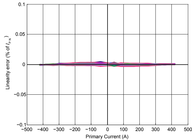
Figure 5: Linearity
