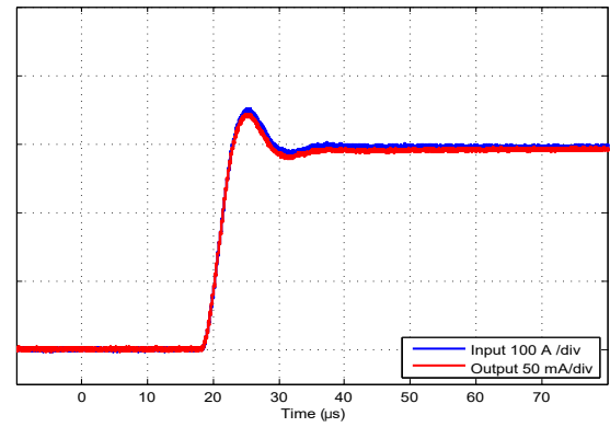
Figure 2: Typical delay time (0 to 300 A, 100 A/μs R_M = 10 \Omega )
