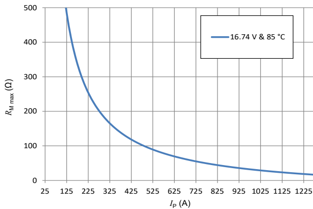
Figure 1: Maximum measuring resistance
