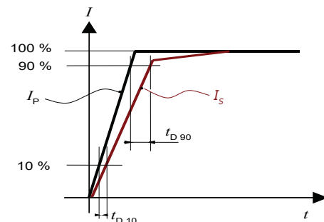
Figure 6: t_{D10} (delay time @ 10 %) and t_{D90} (delay time @ 90 %)
