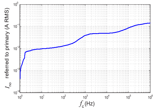
Figure 4: Typical RMS noise current referred to primary I_{no} with R_M = 100 \Omega
