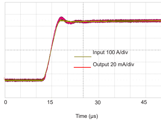
Figure 2: Typical delay time (0 to 500 A, 100 A/ \mu s , R_M = 1 \Omega )
