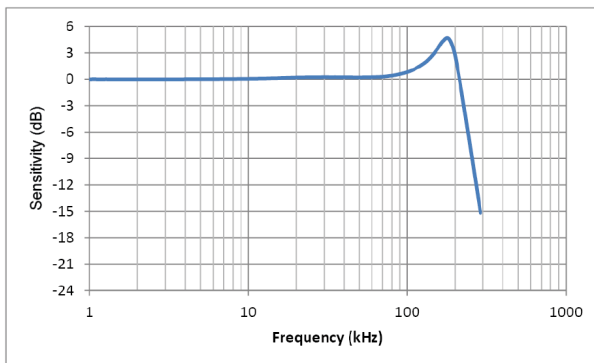
Figure 5: Typical frequency response, small signal bandwidth
