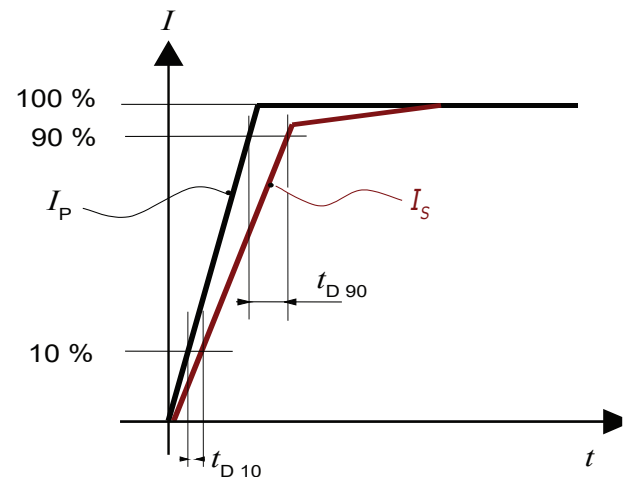
Figure 6: t_{D10} (delay time @ 10 %) and t_{D90} (delay time @ 90 %)
