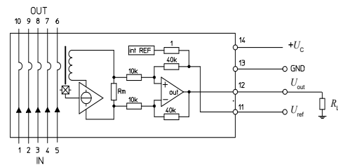
Figure 8: Test connection
