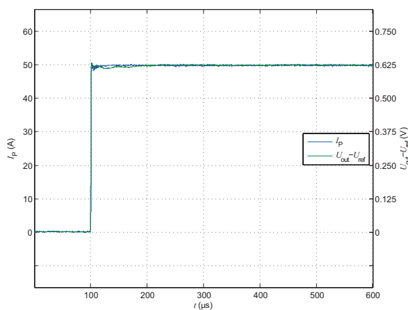
Figure 3: Delay time
