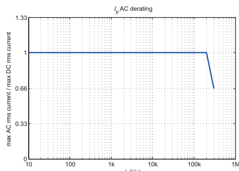
Figure 25: Maximum RMS AC primary current / maximum DC primary current vs frequency
