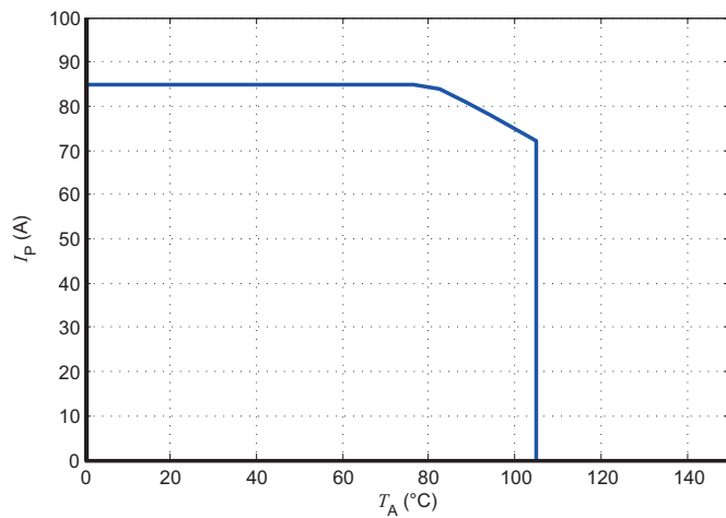
Figure 23: I_P vs T_A for LKSR 25-NP
