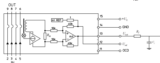
Figure 11: Filtered U_{out} connection
