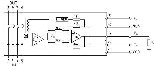
Figure 8: Test connection
