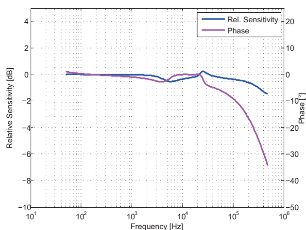
Figure 2: Frequency response
