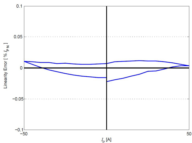
Figure 1: Linearity error
