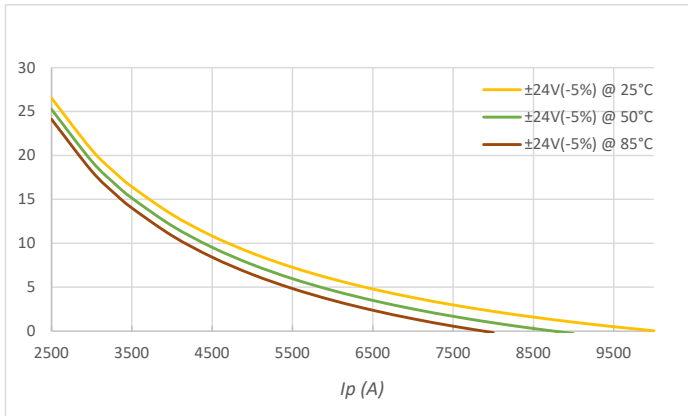
Figure 1: Maximum measuring resistance
