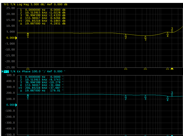
Figure 5: Frequency bandwidth
