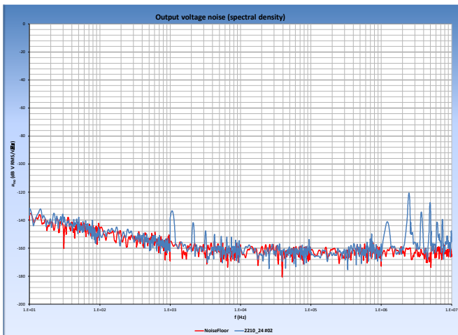
Figure 3: Typical output noise voltage spectral density with R_M = 9 Ohm (test done on LT 4000-S/SP35)
