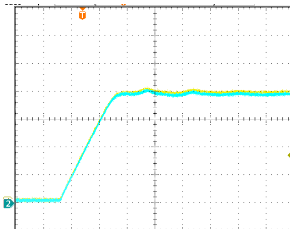
Figure 2: ch1: I_p = 4000 A/div ; ch2: I_s = 0.2 A/div , dI/dt 50 A/\mu s according to the report CA031109 (test done on LT 4000-T/SP42)
