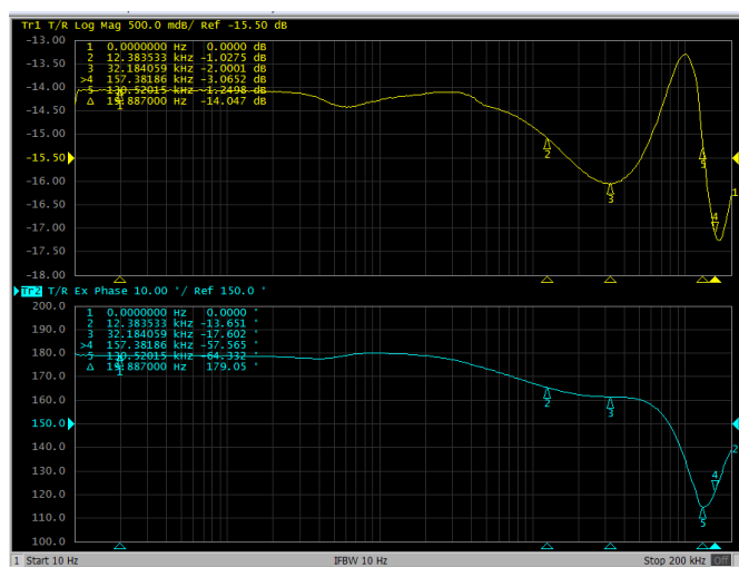
Figure 5: Frequency bandwidth
