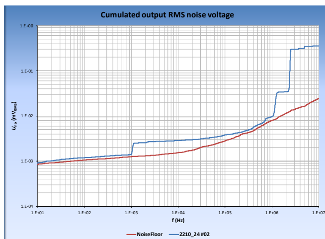
Figure 4: Typical output RMS noise current with R_M = 1 \text{ Ohm} (primary referred) (test done on LT 4000-S/SP35)
