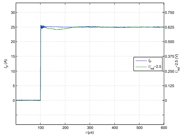
Figure 13: Delay time
