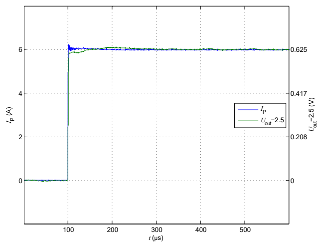
Figure 3: Delay time
