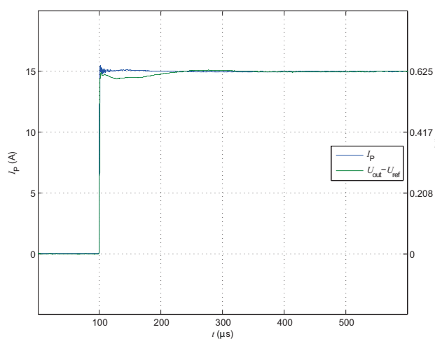
Figure 8: Delay time
