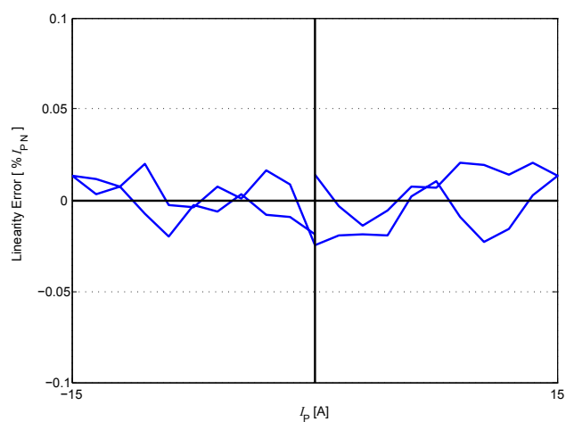
Figure 6: Linearity error
