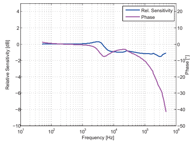
Figure 12: Frequency response
