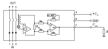
Figure 20: Test connection
