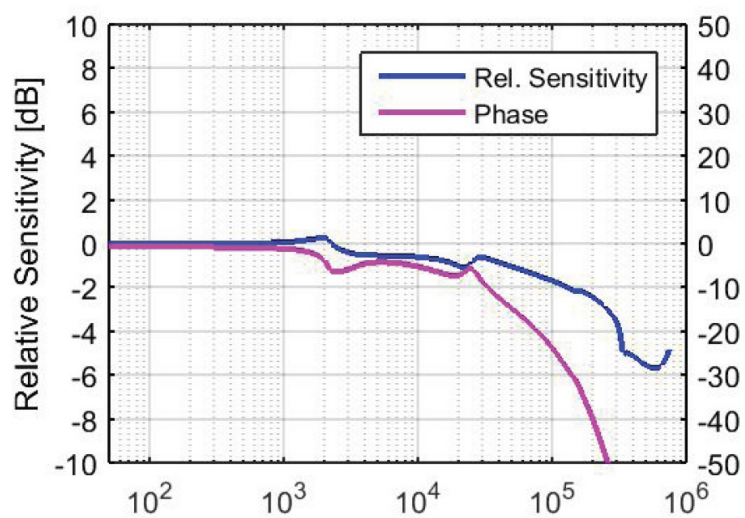
Figure 2: Frequency response
