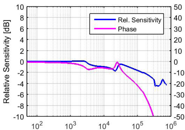
Figure 2: Frequency response
