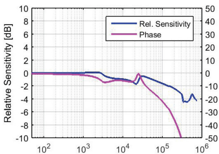
Figure 2: Frequency response
